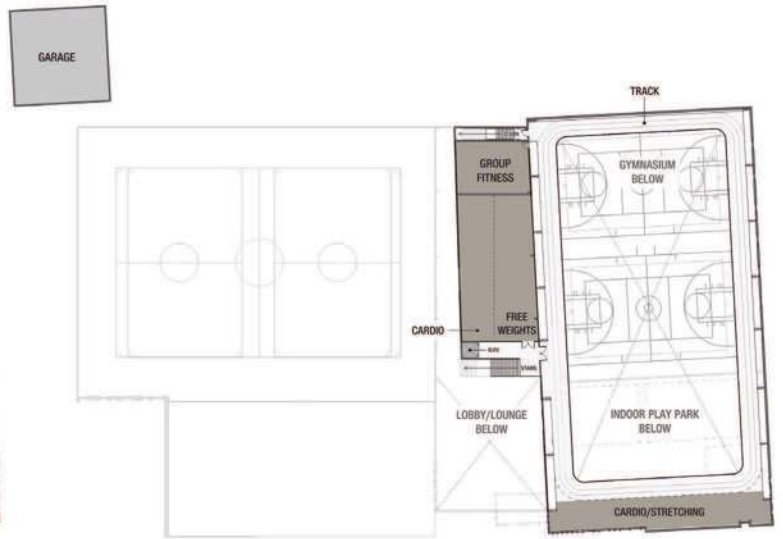
Phase I - Second Floor Plan
